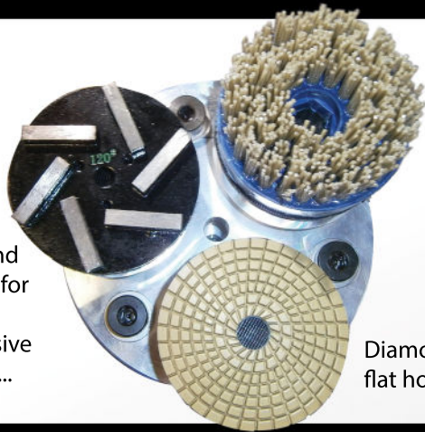
PadHead Model II on a grinder for flat polishing or honing
