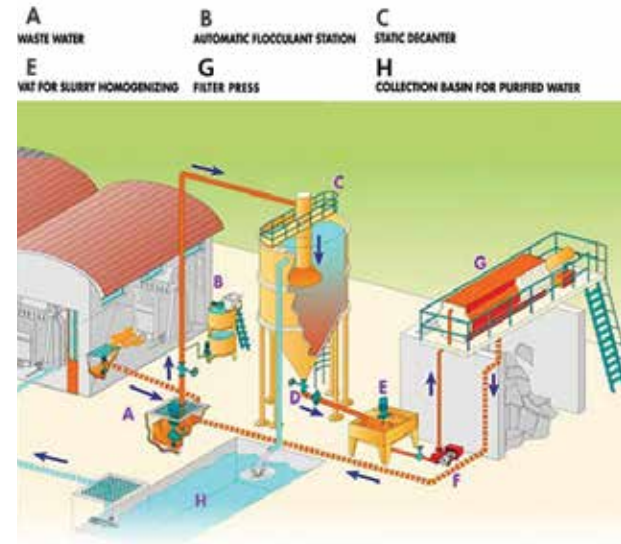
Water Treatment Plants by F&B Separates the waste product & water; recycled water returns for use. Systems eliminate sludge pits/monthly cleaning.
